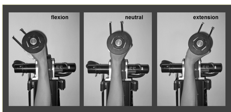
Figure 1 Forearm and hand position in the robotic wrist device (upper view). The forearm rests in a cushioned support in mid pronation-supination. The axis of rotation of the wrist is aligned with the axis of the device. The fingers were lightly fixed around the handle and supported with a velcro strap. The robotic device moves the wrist in a cyclic manner through flexion and extension with a smooth sinusoidal velocity profile. Movement is restricted to only the flexion-extension (sagittal) plane.
