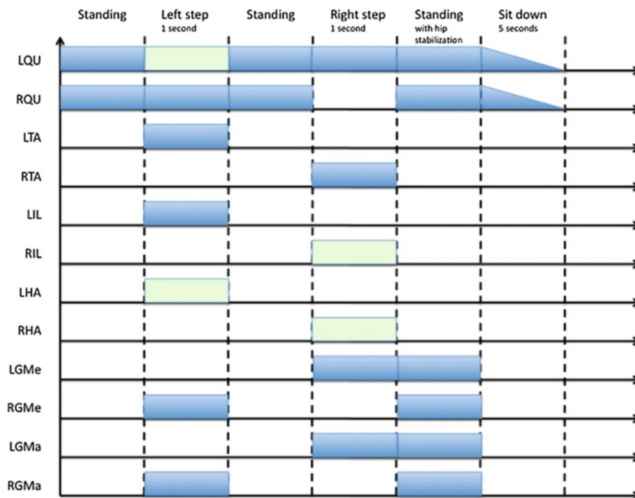
Figure 2 Sequences of stimulation required for a full step and used for gait assessment. Stimulation amplitude is not represented because it depends on muscle fatigue and individual features. The green rectangles show facultative muscle contractions that improve the comfort of the patient but not the performances
