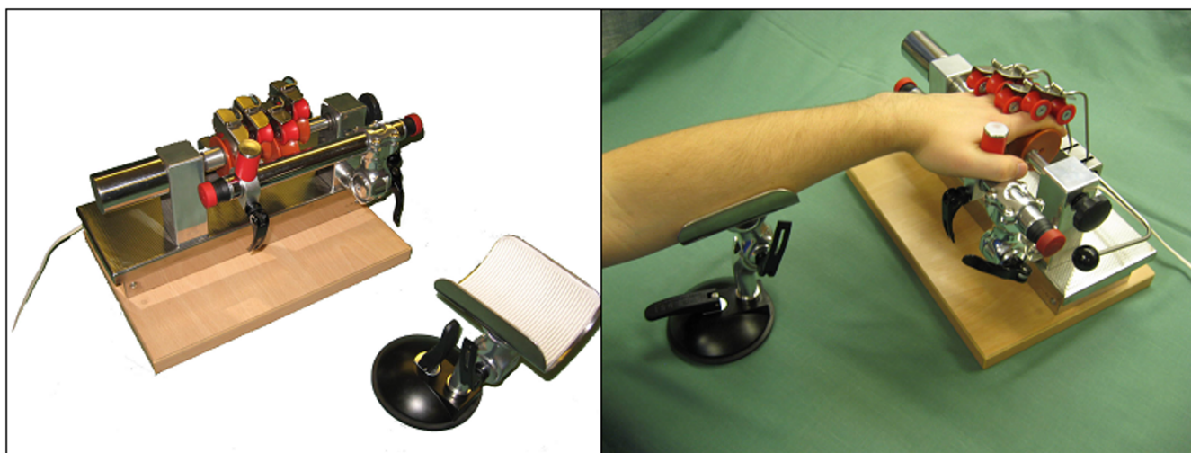
Figure 1 The Finger Trainer, "Reha-Digit", without a patient (left), and a left-hemiparetic patient practicing with the device (right).
