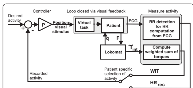
Figure 3 Control scheme for control of activity via a visual stimulus. Active participation is measured by HR or weighted interaction torques (WIT). The control loop is closed by the visual feedback to the patient. T_{int} are the interaction torques between Lokomat and human. If HR control is chosen, mean HR is extracted in real time from the ECG and compared to a desired HR value. If WIT is controlled to a desired value, the current WIT values are computed from the interaction torques as detailed in the section ‘Quantifying patient participation’ and in Banz et al. [20]. The position of the visual stimulus is computed with a P gain.
